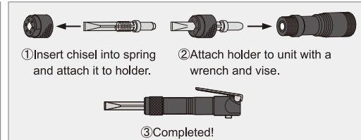
NFB-25H (Slide Ball Retainer)
